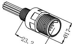
Ultra small 16 core male seat SFCXZBH16M
