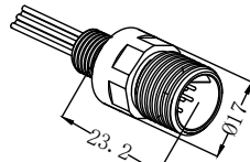
Ultra small 12 core male seat SFCXZBH12M
