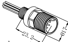
Ultra small 8 core male seat SFCXZBH8M
